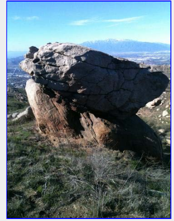
Gneiss shouldered by Granite on Box Springs Mt, Moreno Valley CA [William Wright photo]
